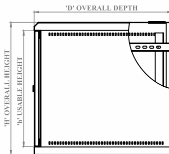
SIDE VIEW-RHS
