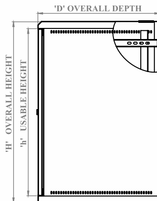
SIDE VIEW-RHS
